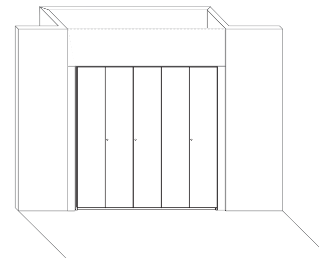
04 Armadio in nicchia con chiusure laterali e superiori Wardrobe in recess with horizontal and lateral fillers
