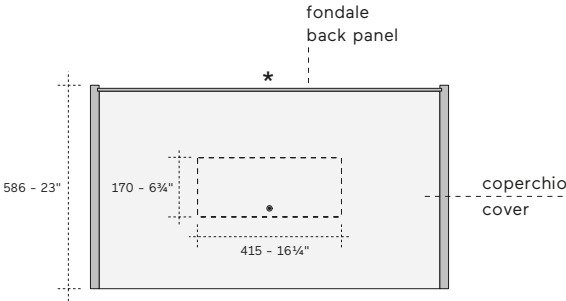
Vista pianta Plan view
